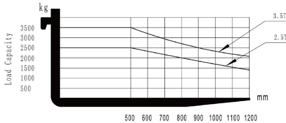
Load Center Load Curve
